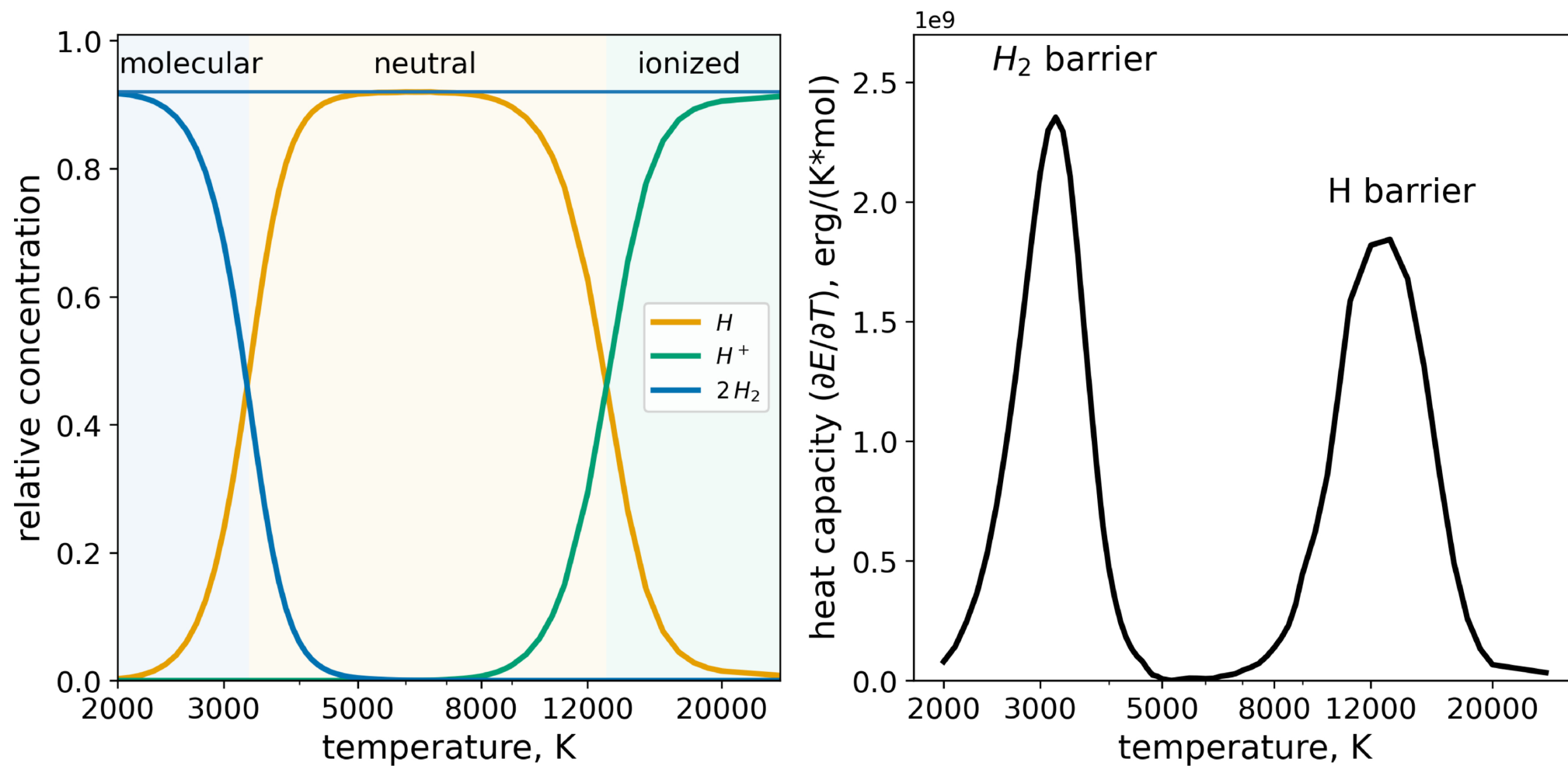
Figure 2. from A. I. Shapiro et al 2026 Astrophys. J. Lett. 998 doi:10.3847/2041-8213/ae328b https://dx.doi.org/10.3847/2041-8213/ae328b © 2026. The Author(s). Published by the American Astronomical Society.
