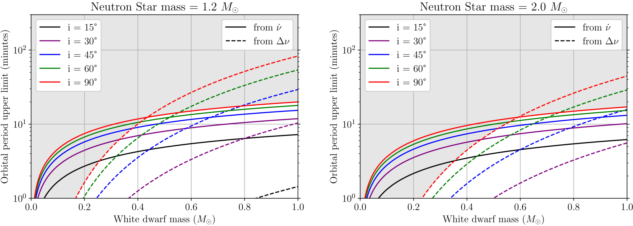
Figure 5. from Sébastien Le Stum et al 2026 Astrophys. J. Lett. 997 doi:10.3847/2041-8213/ae3174 https://dx.doi.org/10.3847/2041-8213/ae3174 © 2026. The Author(s). Published by the American Astronomical Society.
