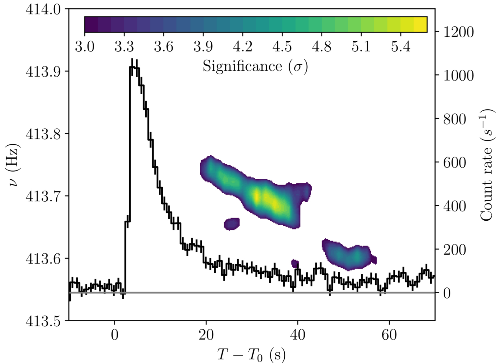
Figure 3. from Sébastien Le Stum et al 2026 Astrophys. J. Lett. 997 doi:10.3847/2041-8213/ae3174 https://dx.doi.org/10.3847/2041-8213/ae3174 © 2026. The Author(s). Published by the American Astronomical Society.
