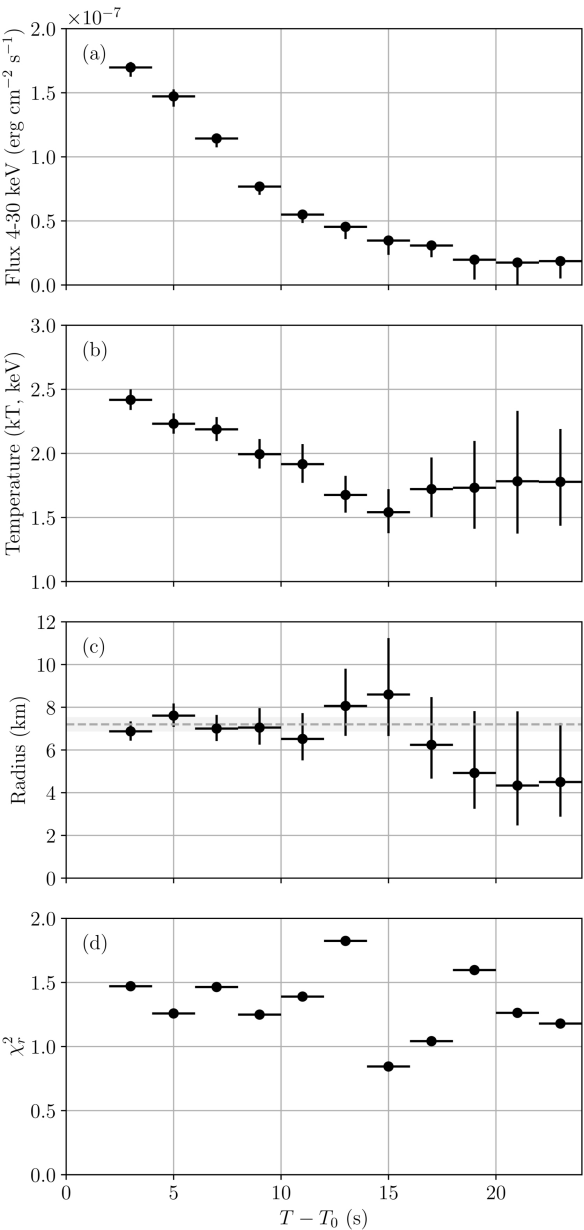
Figure 2. from Sébastien Le Stum et al 2026 Astrophys. J. Lett. 997 doi:10.3847/2041-8213/ae3174 https://dx.doi.org/10.3847/2041-8213/ae3174 © 2026. The Author(s). Published by the American Astronomical Society.
