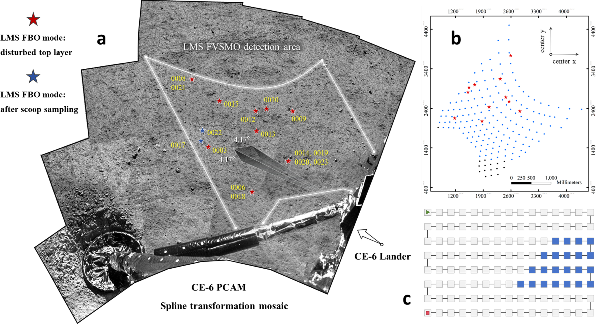
Figure A2. from Siyue Chi et al 2026 Astrophys. J. Lett. 997 doi:10.3847/2041-8213/ae3166 https://dx.doi.org/10.3847/2041-8213/ae3166 © 2026. The Author(s). Published by the American Astronomical Society.
