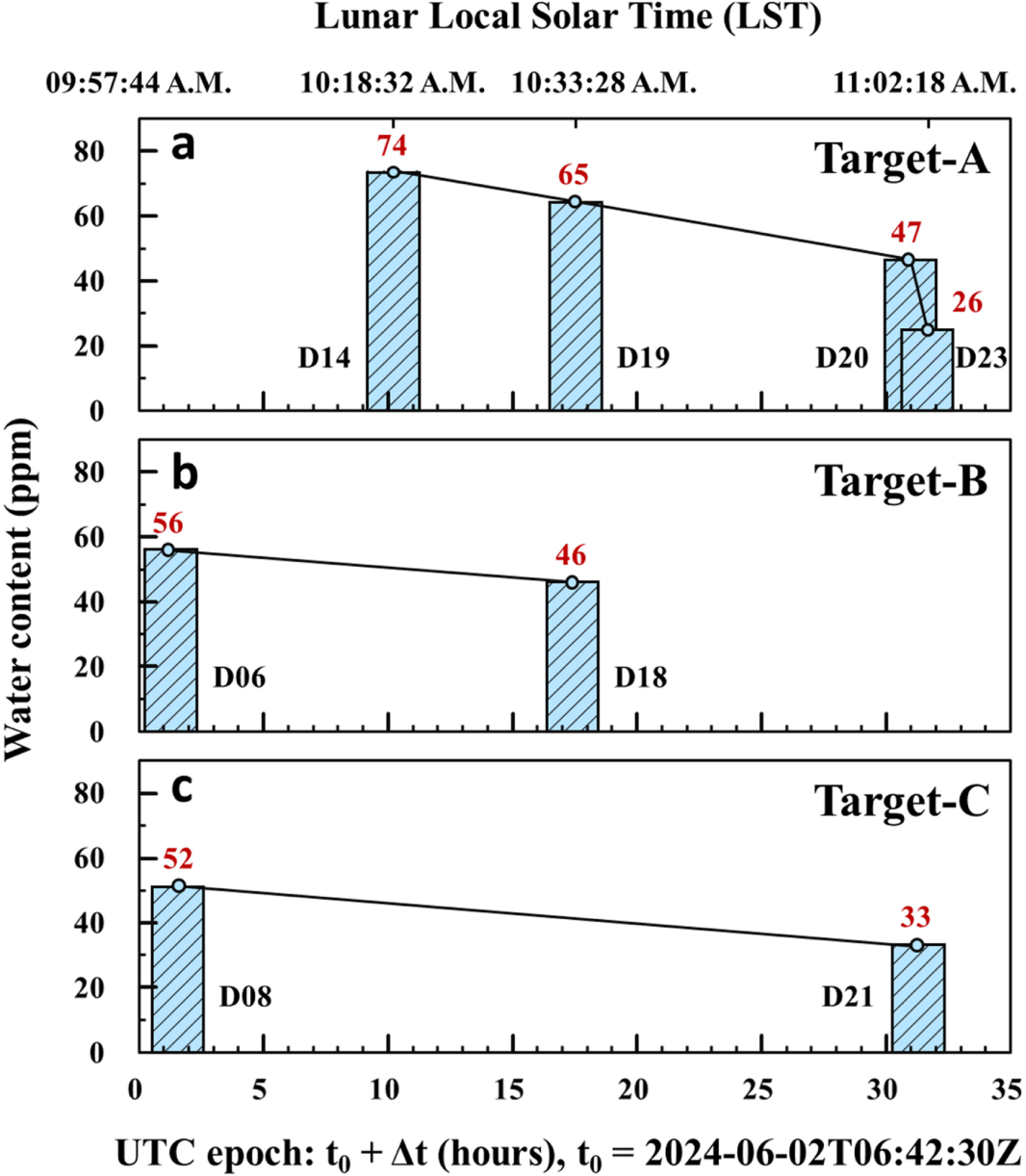
Figure 3. from Siyue Chi et al 2026 Astrophys. J. Lett. 997 doi:10.3847/2041-8213/ae3166 https://dx.doi.org/10.3847/2041-8213/ae3166 © 2026. The Author(s). Published by the American Astronomical Society.
