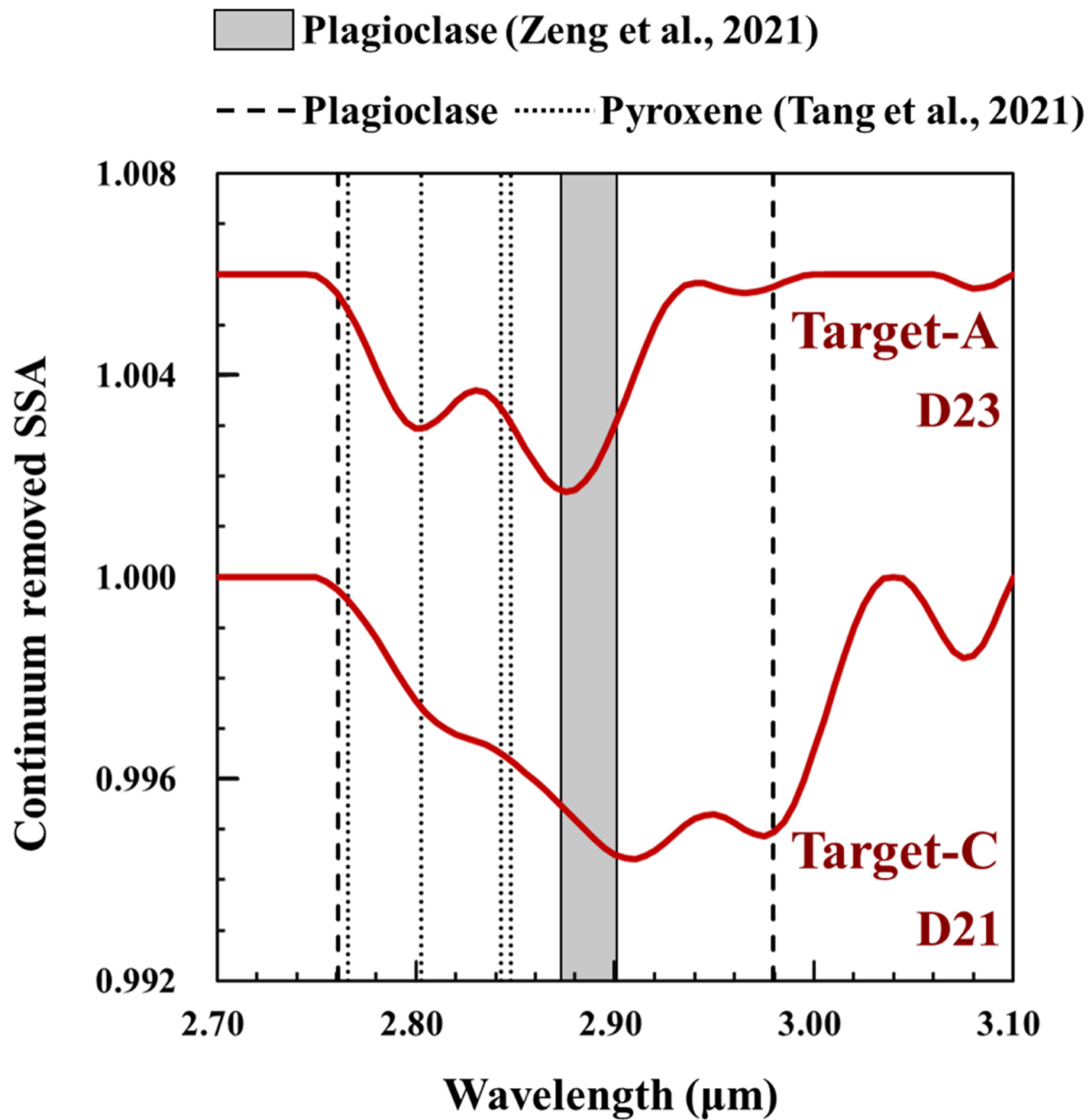
Figure 2. from Siyue Chi et al 2026 Astrophys. J. Lett. 997 doi:10.3847/2041-8213/ae3166 https://dx.doi.org/10.3847/2041-8213/ae3166 © 2026. The Author(s). Published by the American Astronomical Society.
