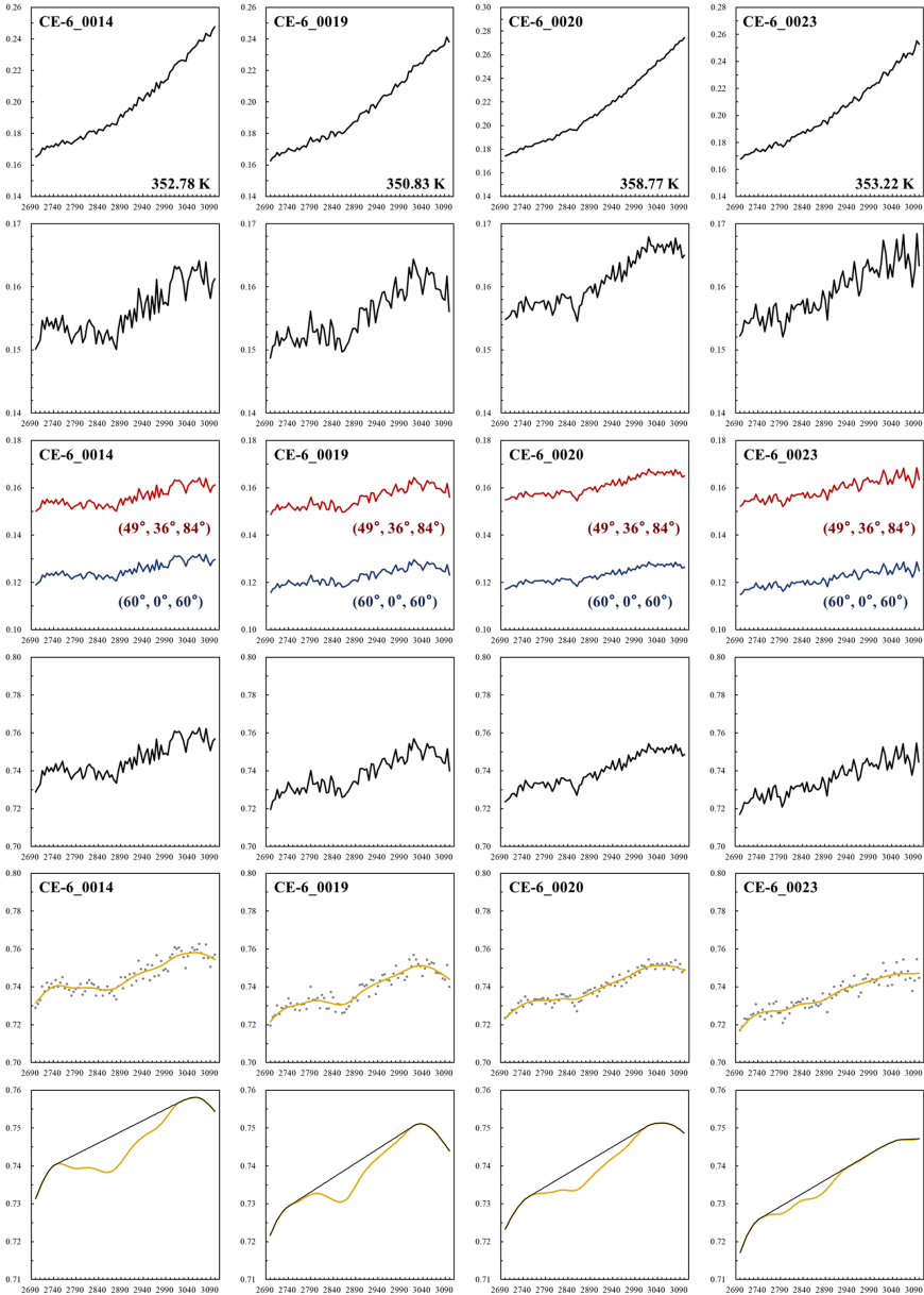
Figure A6. from Siyue Chi et al 2026 Astrophys. J. Lett. 997 doi:10.3847/2041-8213/ae3166 https://dx.doi.org/10.3847/2041-8213/ae3166 © 2026. The Author(s). Published by the American Astronomical Society.
