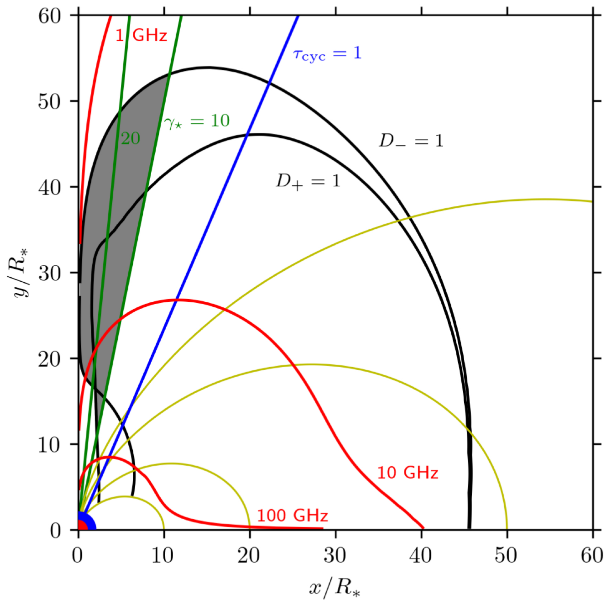
Figure 6. from Shuzhe Zeng et al 2026 Astrophys. J. Lett. 996 doi:10.3847/2041-8213/ae2ade https://dx.doi.org/10.3847/2041-8213/ae2ade © 2025. The Author(s). Published by the American Astronomical Society.
