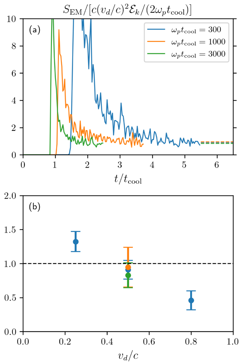
Figure 5. from Shuzhe Zeng et al 2026 Astrophys. J. Lett. 996 doi:10.3847/2041-8213/ae2ade https://dx.doi.org/10.3847/2041-8213/ae2ade © 2025. The Author(s). Published by the American Astronomical Society.
