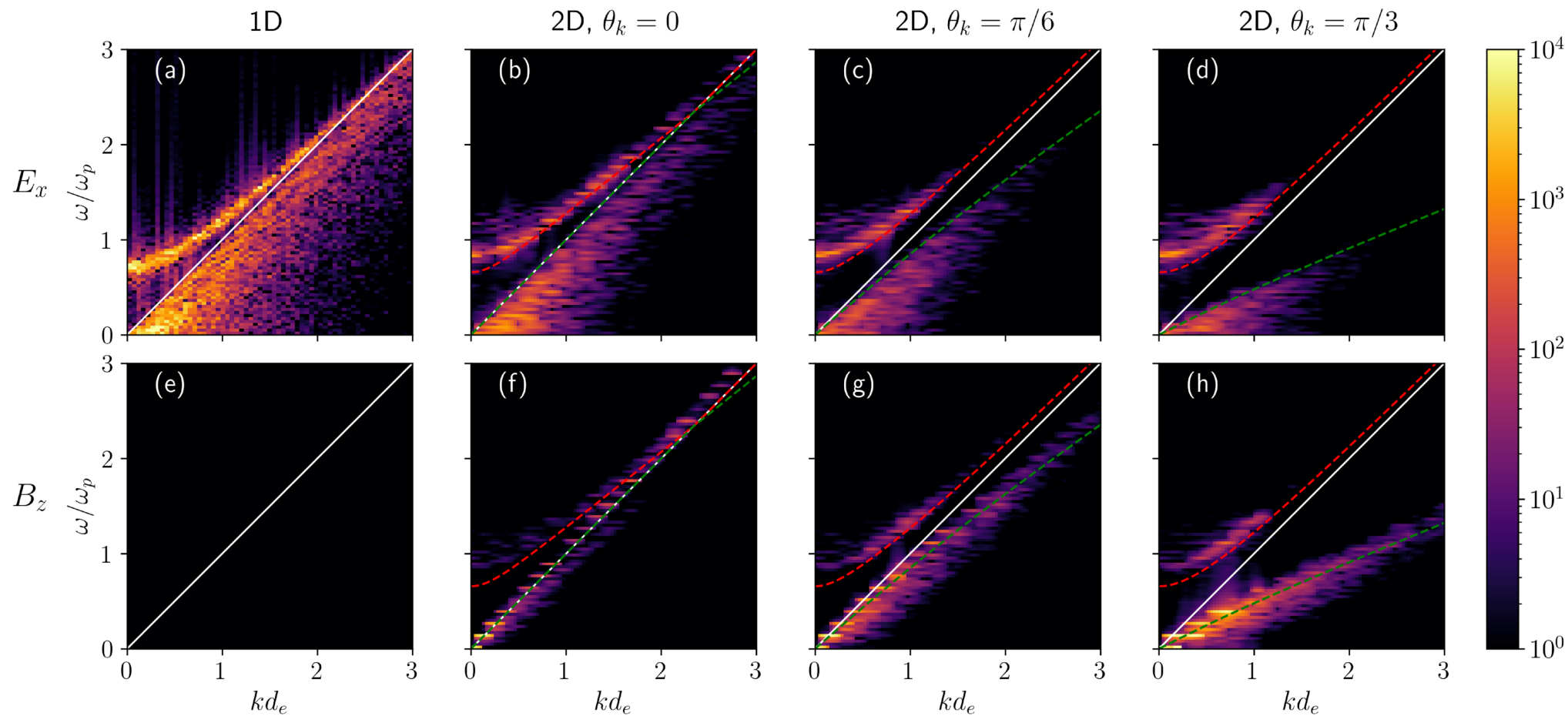
Figure 4. from Shuzhe Zeng et al 2026 Astrophys. J. Lett. 996 doi:10.3847/2041-8213/ae2ade https://dx.doi.org/10.3847/2041-8213/ae2ade © 2025. The Author(s). Published by the American Astronomical Society.
