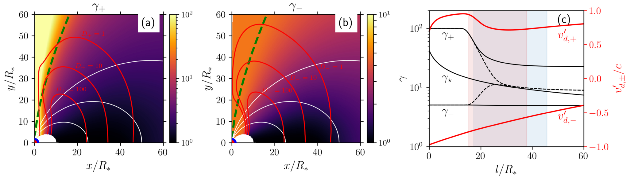
Figure 1. from Shuzhe Zeng et al 2026 Astrophys. J. Lett. 996 doi:10.3847/2041-8213/ae2ade https://dx.doi.org/10.3847/2041-8213/ae2ade © 2025. The Author(s). Published by the American Astronomical Society.
