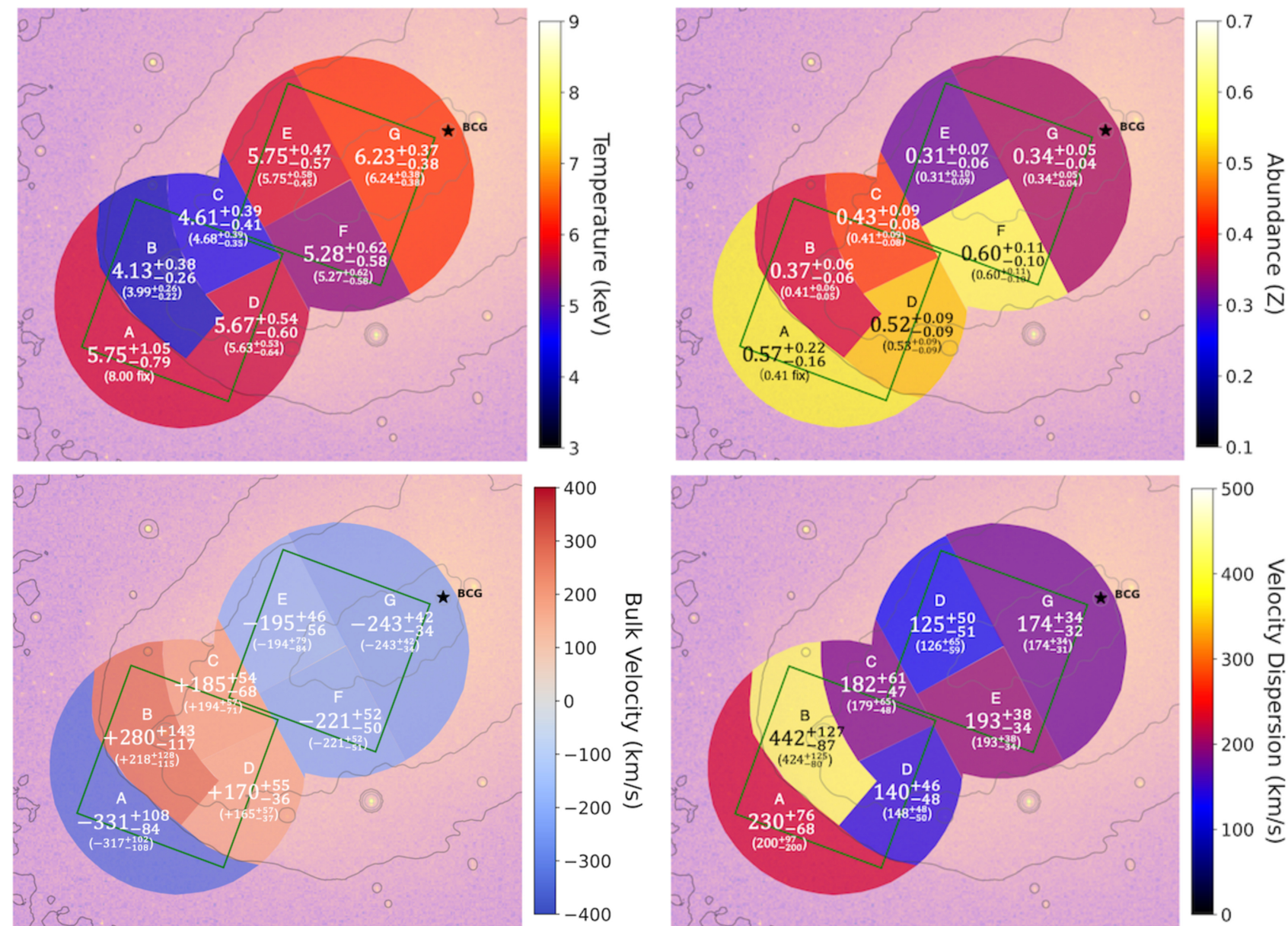
Figure 5. from Yuki Omiya et al 2026 Astrophys. J. Lett. 996 doi:10.3847/2041-8213/ae2a28 https://dx.doi.org/10.3847/2041-8213/ae2a28 © 2025. The Author(s). Published by the American Astronomical Society.
