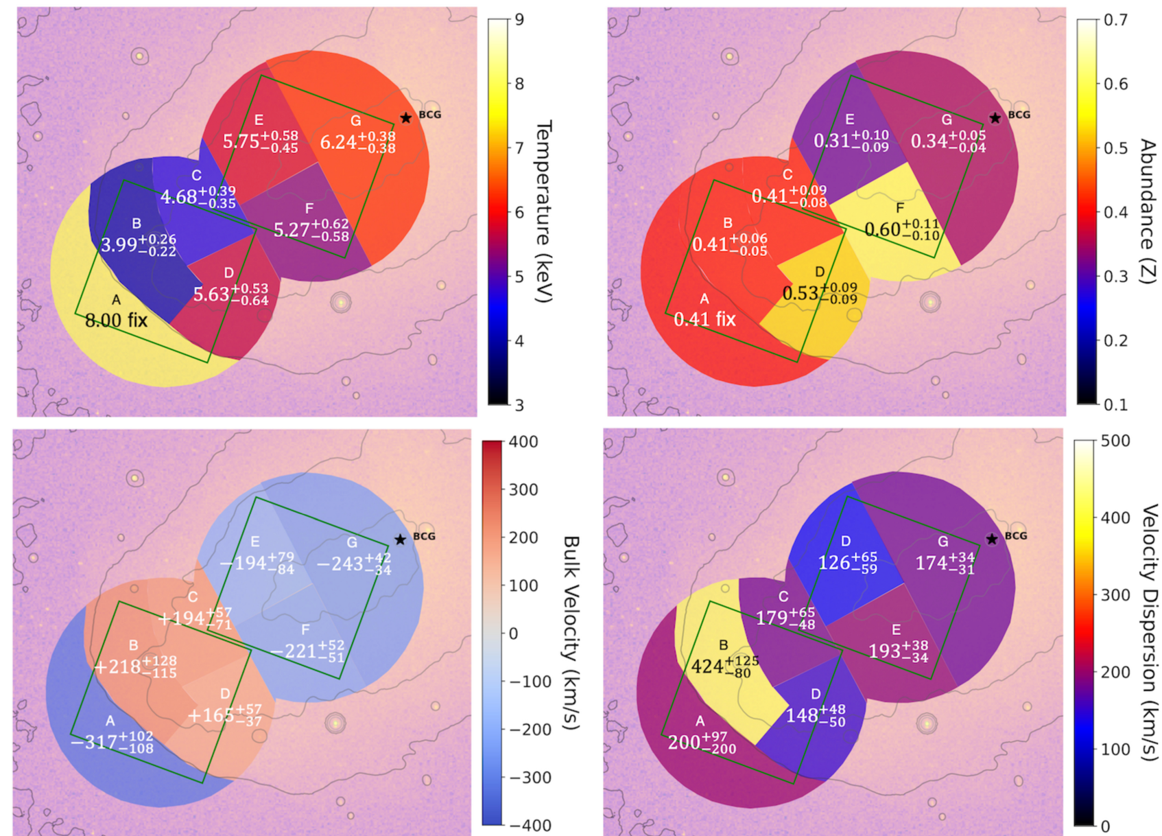
Figure 3. from Yuki Omiya et al 2026 Astrophys. J. Lett. 996 doi:10.3847/2041-8213/ae2a28 https://dx.doi.org/10.3847/2041-8213/ae2a28 © 2025. The Author(s). Published by the American Astronomical Society.
