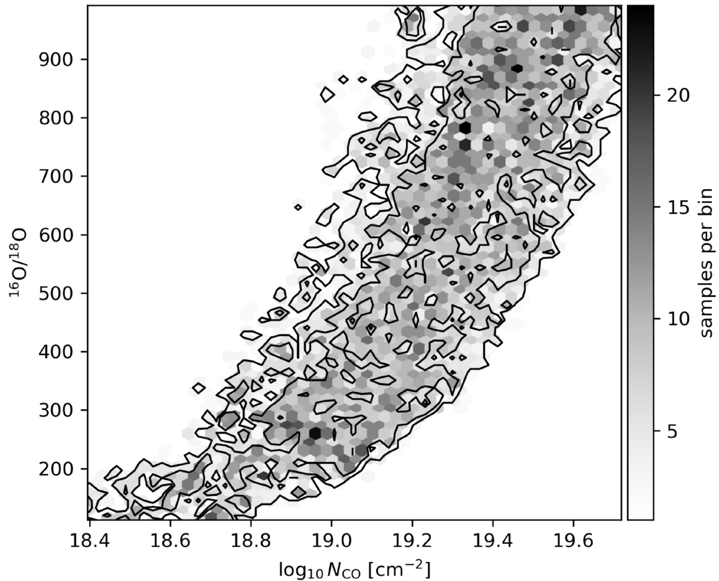
Figure 8. from Chunhua Qi et al 2026 Astrophys. J. Lett. 997 doi:10.3847/2041-8213/ae2916 https://dx.doi.org/10.3847/2041-8213/ae2916 © 2026. The Author(s). Published by the American Astronomical Society.
