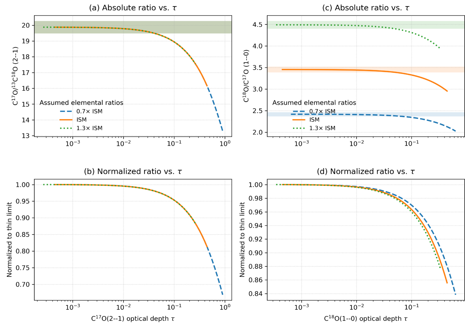
Sensitivity of ratio- \tau curves to assumed isotope ratios
