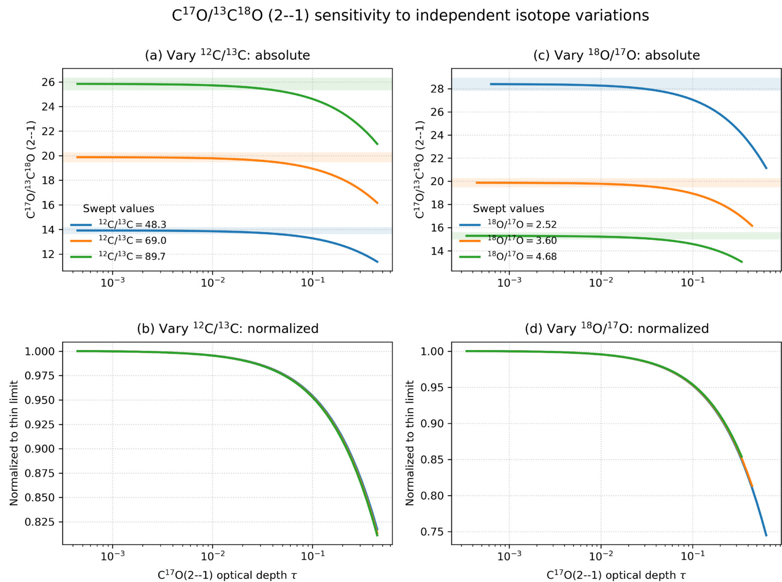
Figure 5. from Chunhua Qi et al 2026 Astrophys. J. Lett. 997 doi:10.3847/2041-8213/ae2916 https://dx.doi.org/10.3847/2041-8213/ae2916 © 2026. The Author(s). Published by the American Astronomical Society.
