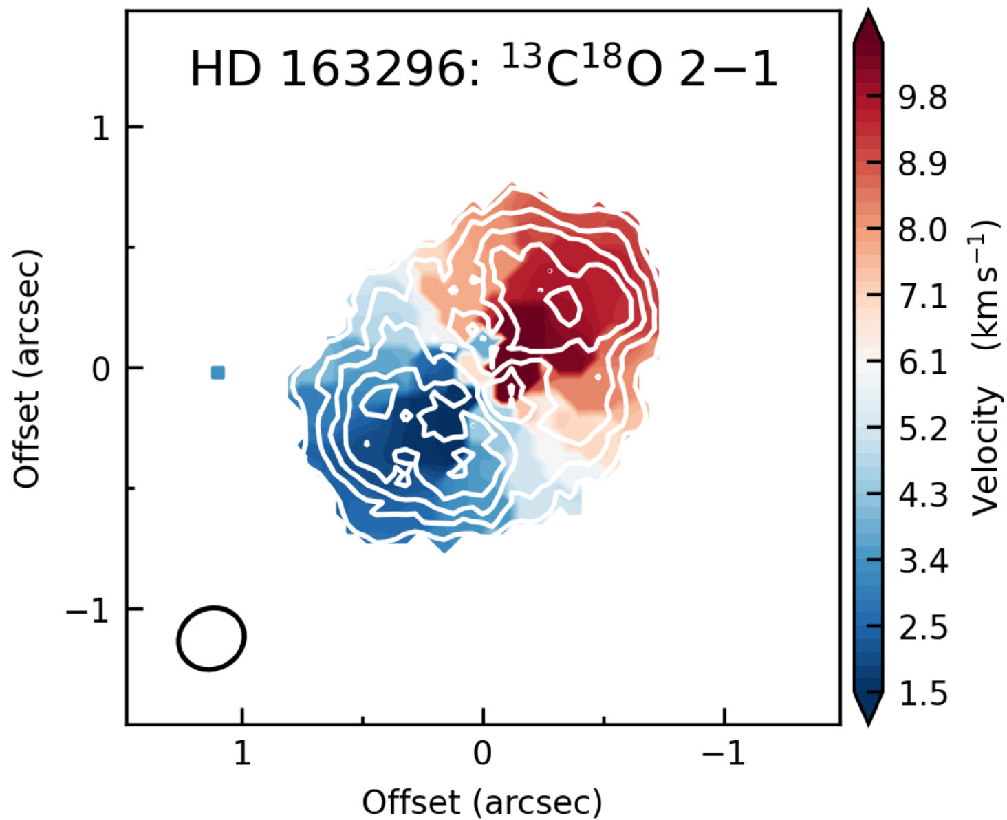
Figure 4. from Chunhua Qi et al 2026 Astrophys. J. Lett. 997 doi:10.3847/2041-8213/ae2916 https://dx.doi.org/10.3847/2041-8213/ae2916 © 2026. The Author(s). Published by the American Astronomical Society.
