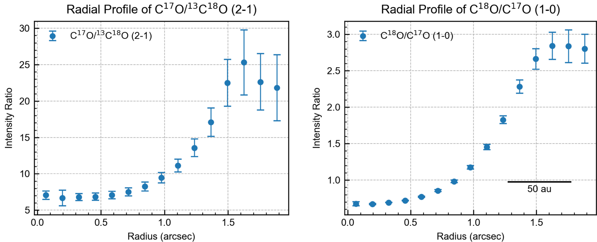
Figure 2. from Chunhua Qi et al 2026 Astrophys. J. Lett. 997 doi:10.3847/2041-8213/ae2916 https://dx.doi.org/10.3847/2041-8213/ae2916 © 2026. The Author(s). Published by the American Astronomical Society.
