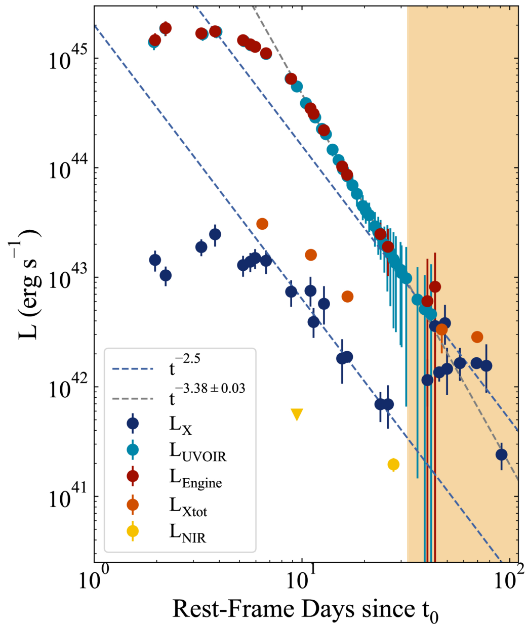
Figure 8. from Natalie LeBaron et al 2026 Astrophys. J. Lett. 997 doi:10.3847/2041-8213/ae2910 https://dx.doi.org/10.3847/2041-8213/ae2910 © 2026. The Author(s). Published by the American Astronomical Society.
