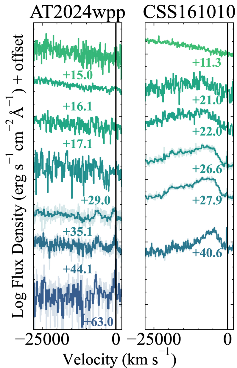
Figure 7. from Natalie LeBaron et al 2026 Astrophys. J. Lett. 997 doi:10.3847/2041-8213/ae2910 https://dx.doi.org/10.3847/2041-8213/ae2910 © 2026. The Author(s). Published by the American Astronomical Society.
