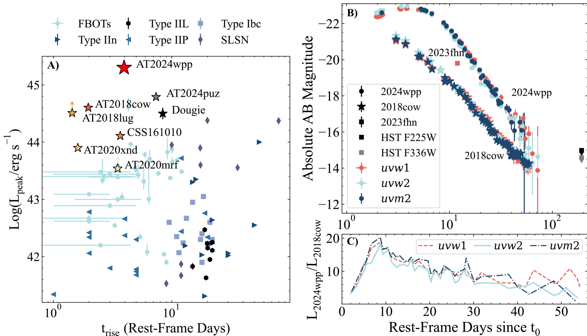
Figure 4. from Natalie LeBaron et al 2026 Astrophys. J. Lett. 997 doi:10.3847/2041-8213/ae2910 https://dx.doi.org/10.3847/2041-8213/ae2910 © 2026. The Author(s). Published by the American Astronomical Society.
