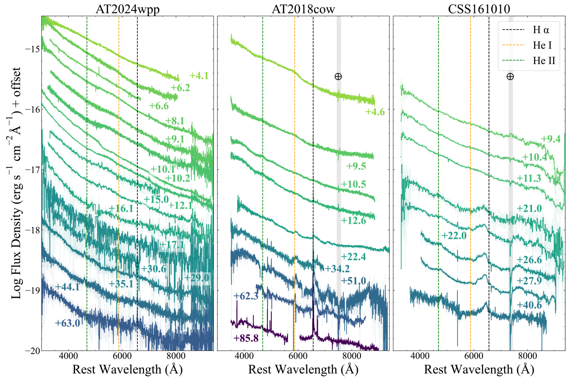
Figure 2. from Natalie LeBaron et al 2026 Astrophys. J. Lett. 997 doi:10.3847/2041-8213/ae2910 https://dx.doi.org/10.3847/2041-8213/ae2910 © 2026. The Author(s). Published by the American Astronomical Society.
