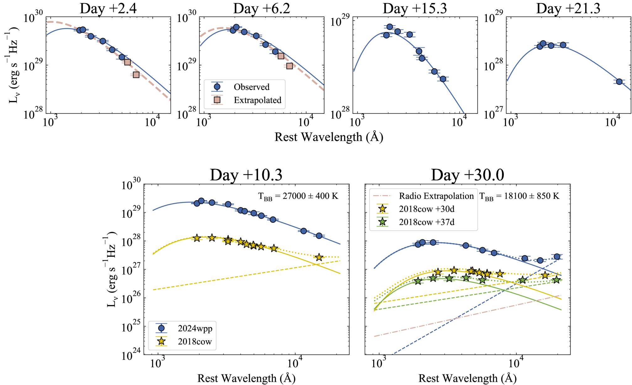
Figure 12. from Natalie LeBaron et al 2026 Astrophys. J. Lett. 997 doi:10.3847/2041-8213/ae2910 https://dx.doi.org/10.3847/2041-8213/ae2910 © 2026. The Author(s). Published by the American Astronomical Society.
