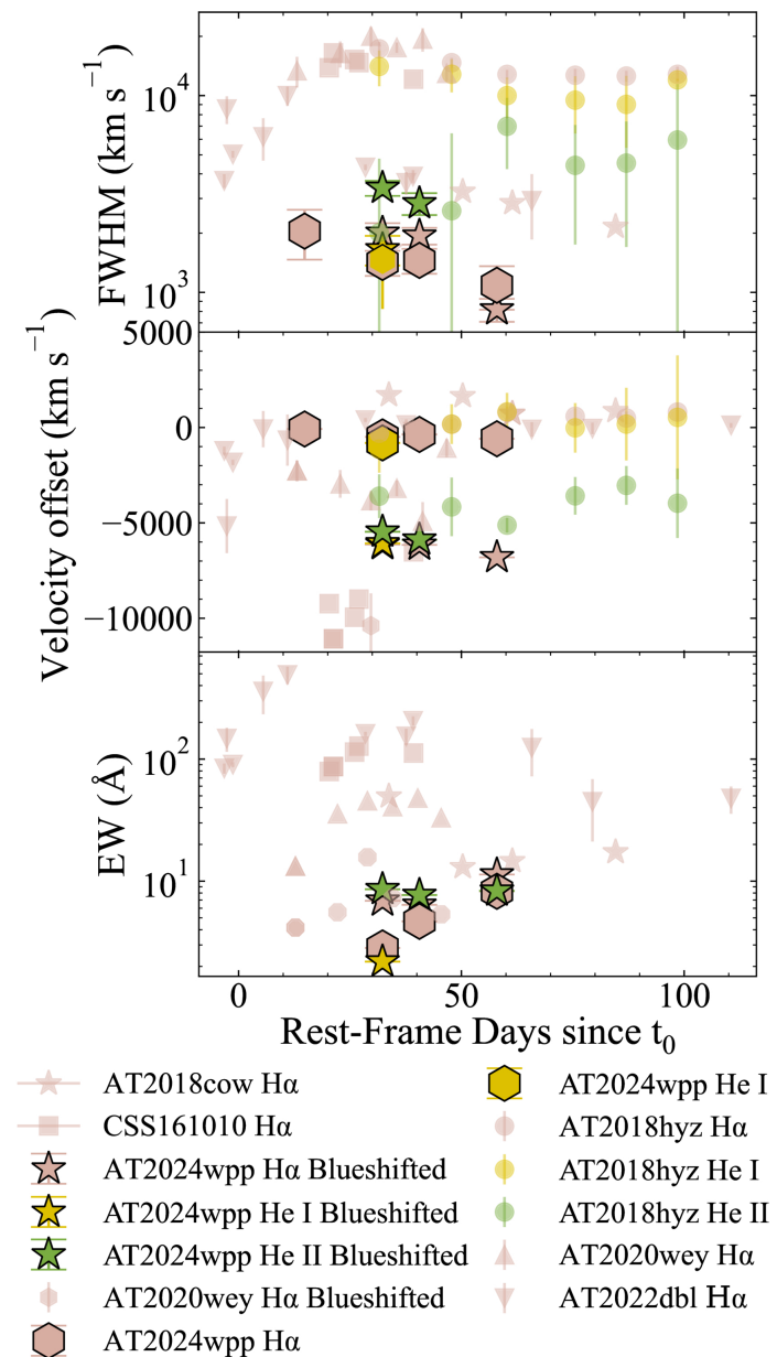
Figure 11. from Natalie LeBaron et al 2026 Astrophys. J. Lett. 997 doi:10.3847/2041-8213/ae2910 https://dx.doi.org/10.3847/2041-8213/ae2910 © 2026. The Author(s). Published by the American Astronomical Society.
