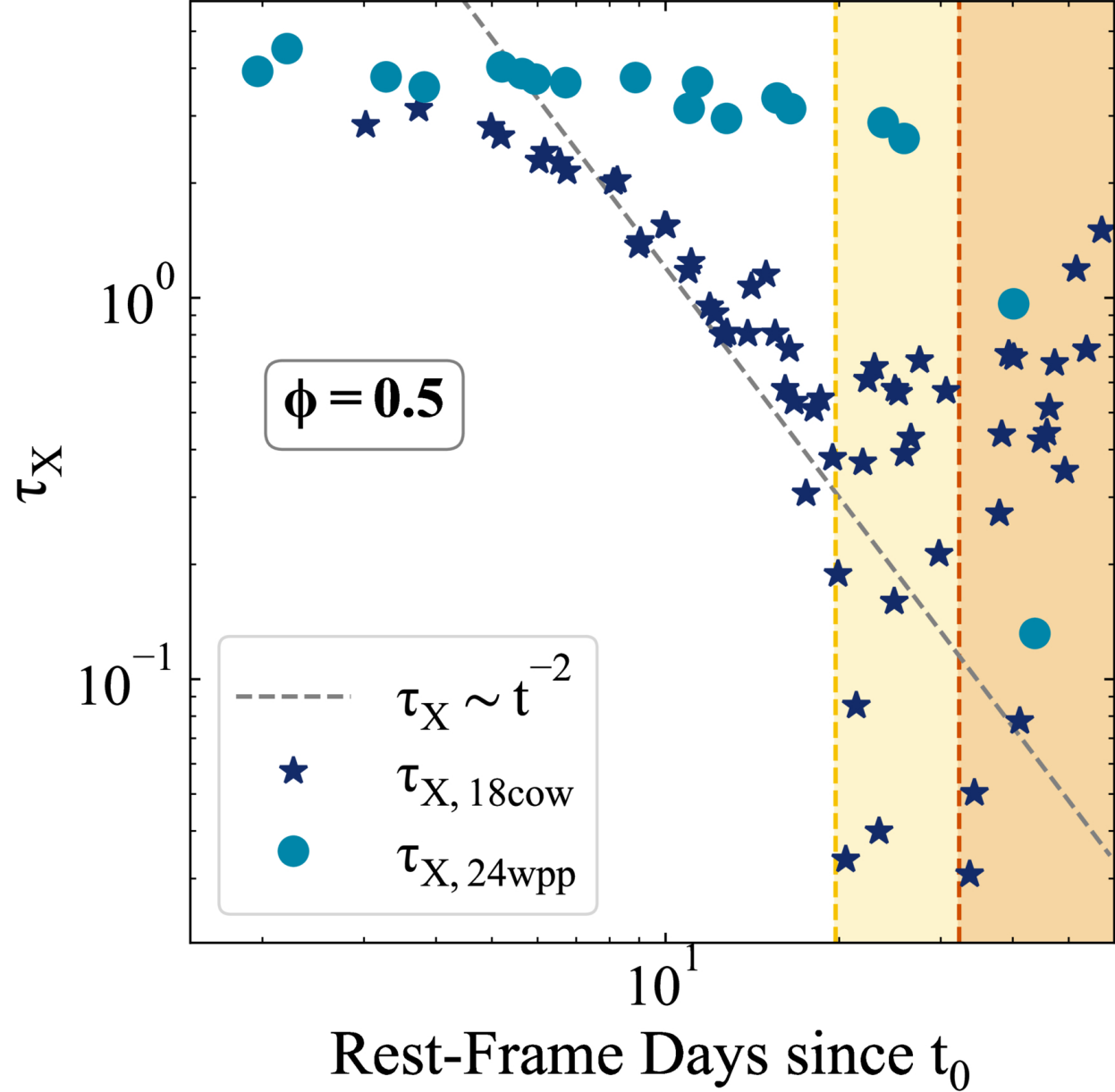
Figure 10. from Natalie LeBaron et al 2026 Astrophys. J. Lett. 997 doi:10.3847/2041-8213/ae2910 https://dx.doi.org/10.3847/2041-8213/ae2910 © 2026. The Author(s). Published by the American Astronomical Society.
