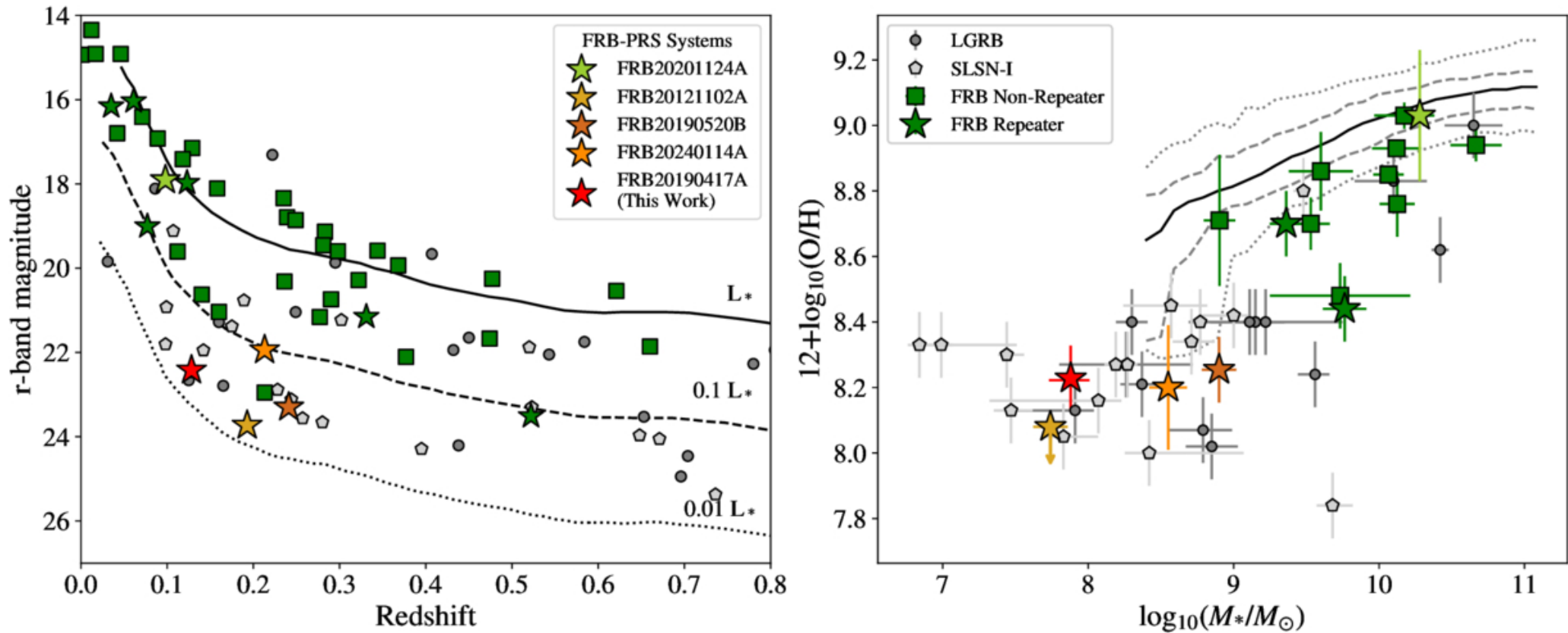
Figure 3. from Alexandra M. Moroianu et al 2026 Astrophys. J. Lett. 996 doi:10.3847/2041-8213/ae28c7 https://dx.doi.org/10.3847/2041-8213/ae28c7 © 2025. The Author(s). Published by the American Astronomical Society.
