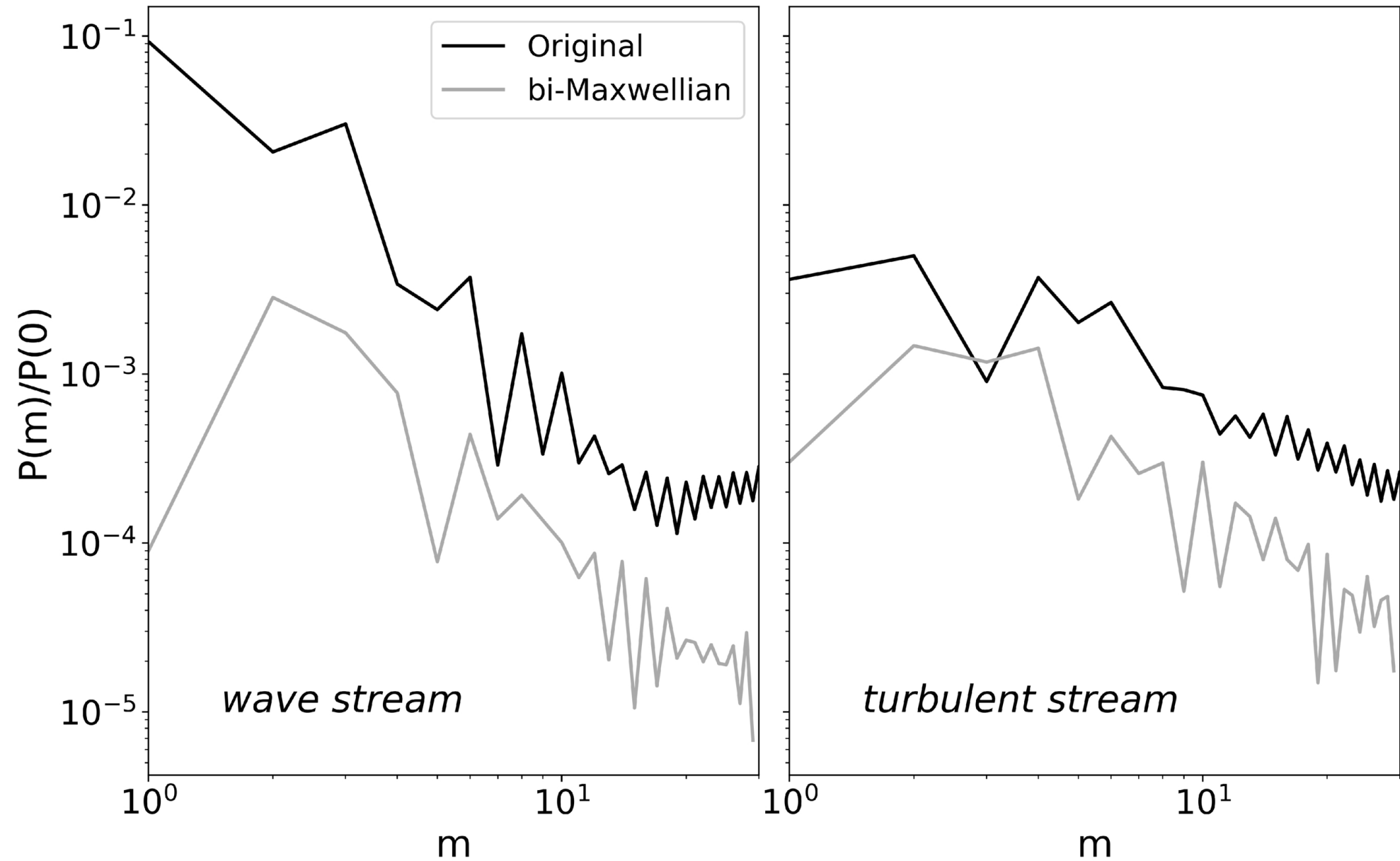
Figure 6. from A. Larosa et al 2025 Astrophys. J. Lett. 995 doi:10.3847/2041-8213/ae2869 https://dx.doi.org/10.3847/2041-8213/ae2869 © 2025. The Author(s). Published by the American Astronomical Society.
