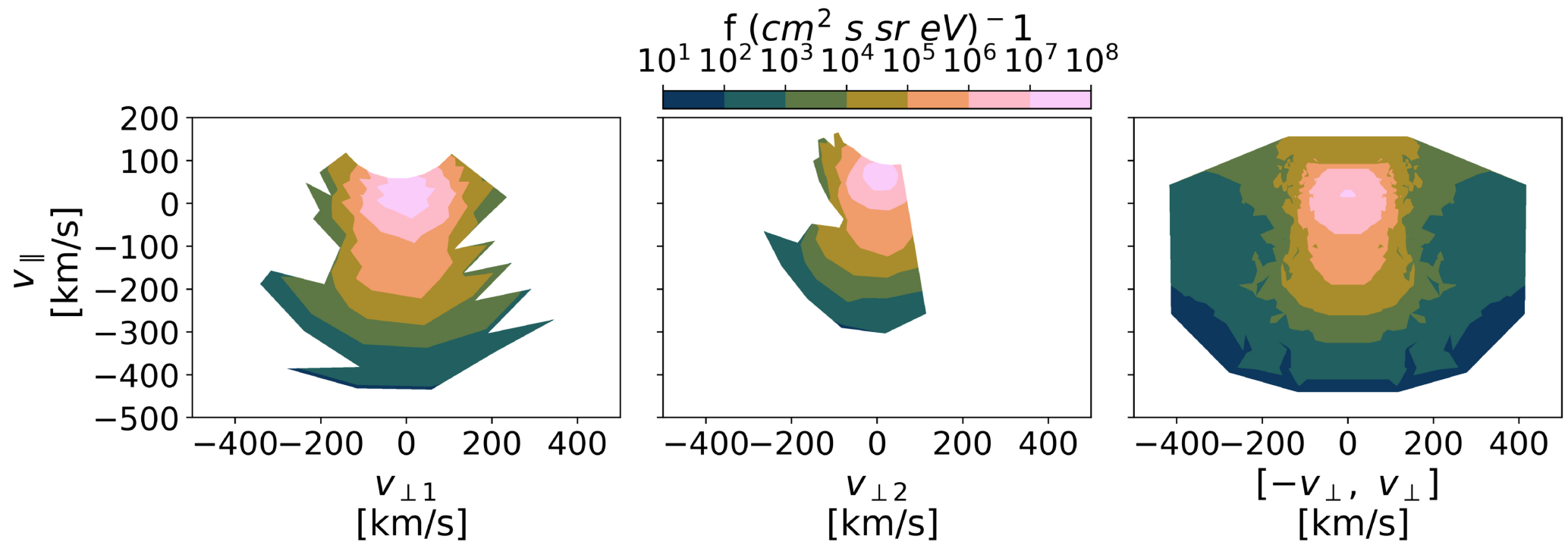
Figure 5. from A. Larosa et al 2025 Astrophys. J. Lett. 995 doi:10.3847/2041-8213/ae2869 https://dx.doi.org/10.3847/2041-8213/ae2869 © 2025. The Author(s). Published by the American Astronomical Society.
