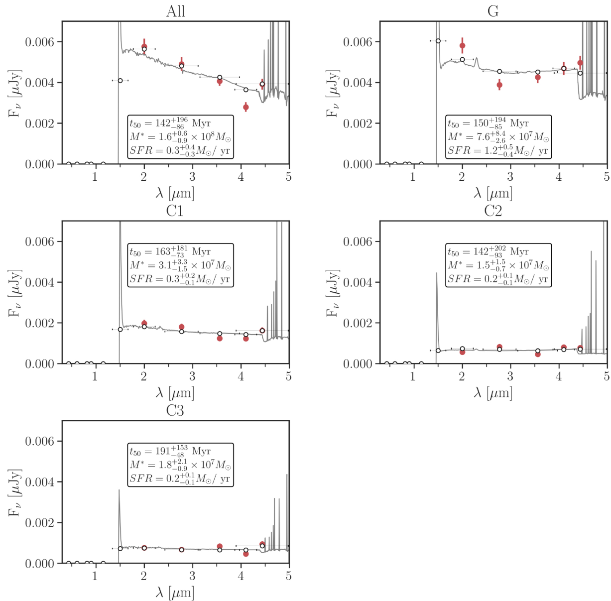
Figure 5. from Maruša Brada et al 2025 Astrophys. J. Lett. 995 doi:10.3847/2041-8213/ae27d2 https://dx.doi.org/10.3847/2041-8213/ae27d2 © 2025. The Author(s). Published by the American Astronomical Society.
