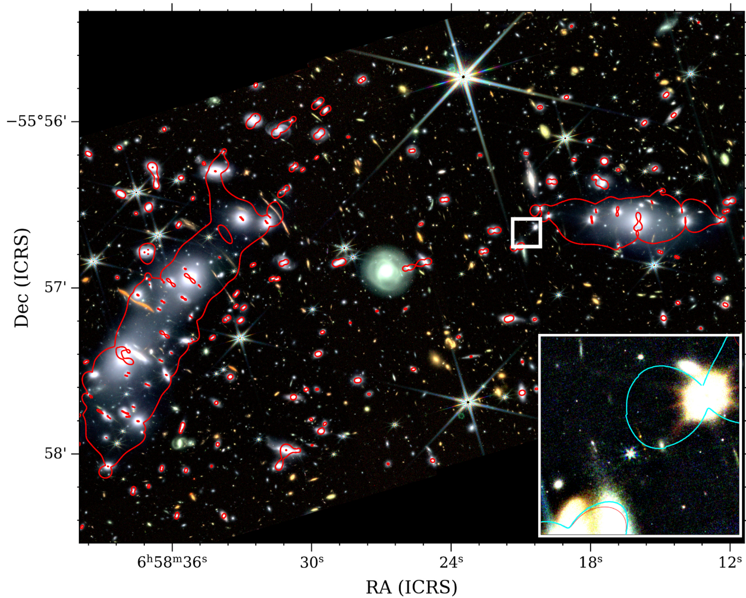
Figure 4. from Maruša Brada et al 2025 Astrophys. J. Lett. 995 doi:10.3847/2041-8213/ae27d2 https://dx.doi.org/10.3847/2041-8213/ae27d2 © 2025. The Author(s). Published by the American Astronomical Society.
