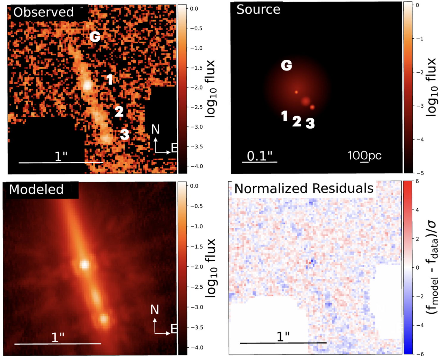
Figure 3. from Maruša Brada et al 2025 Astrophys. J. Lett. 995 doi:10.3847/2041-8213/ae27d2 https://dx.doi.org/10.3847/2041-8213/ae27d2 © 2025. The Author(s). Published by the American Astronomical Society.
