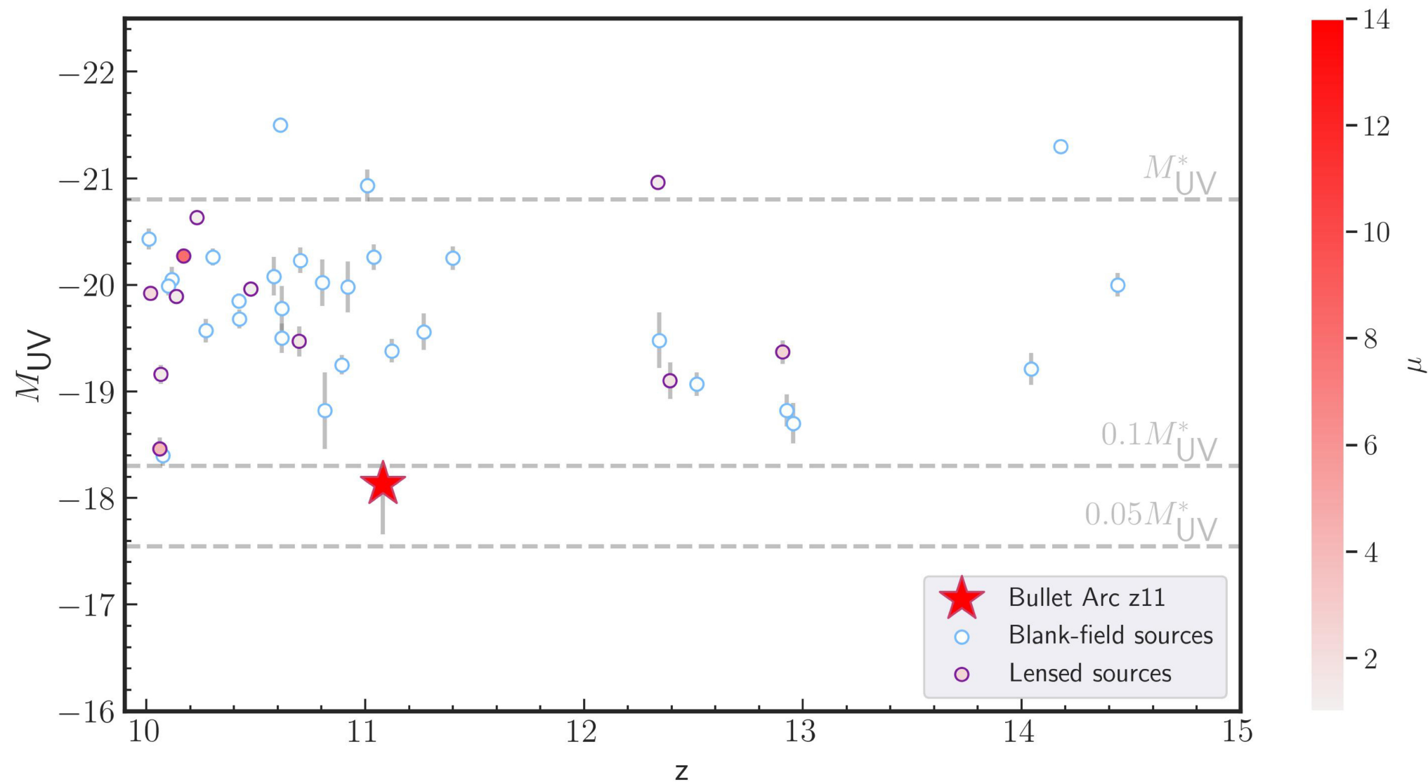
Figure 2. from Maruša Brada et al 2025 Astrophys. J. Lett. 995 doi:10.3847/2041-8213/ae27d2 https://dx.doi.org/10.3847/2041-8213/ae27d2 © 2025. The Author(s). Published by the American Astronomical Society.
