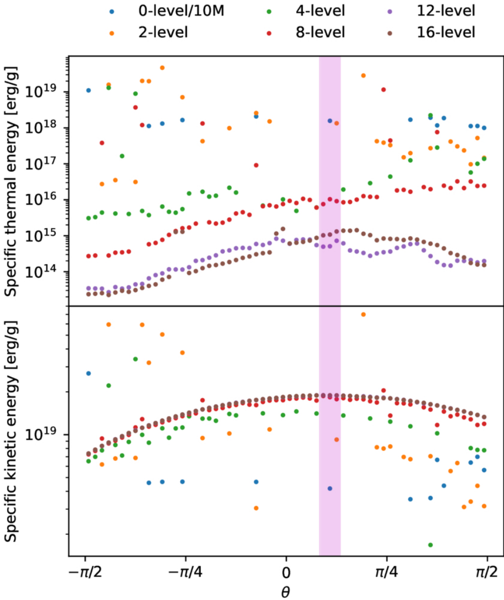
Figure 5. from Fangyi (Fitz) Hu et al 2026 Astrophys. J. Lett. 996 doi:10.3847/2041-8213/ae27cc https://dx.doi.org/10.3847/2041-8213/ae27cc © 2025. The Author(s). Published by the American Astronomical Society.
