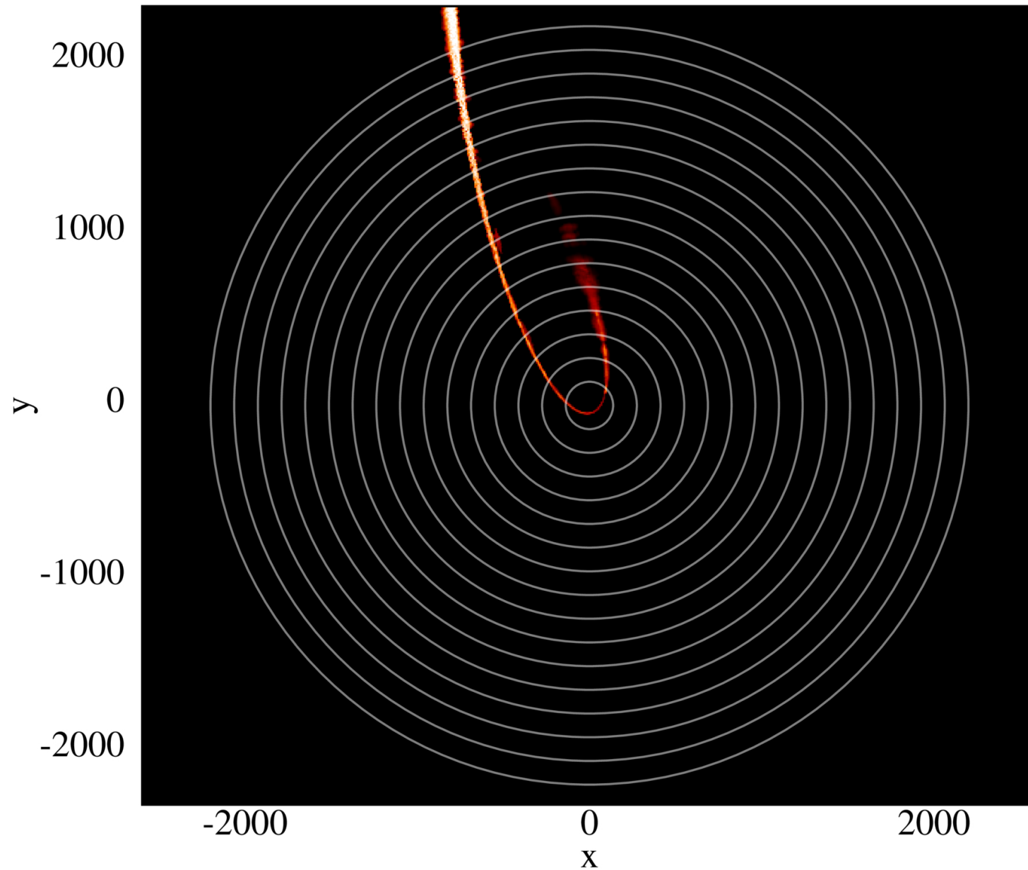
Figure 1. from Fangyi (Fitz) Hu et al 2026 Astrophys. J. Lett. 996 doi:10.3847/2041-8213/ae27cc https://dx.doi.org/10.3847/2041-8213/ae27cc © 2025. The Author(s). Published by the American Astronomical Society.
