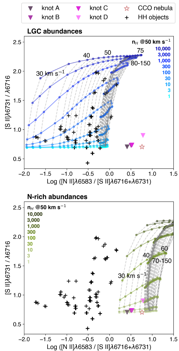
Figure 5. from Janette Suherli et al 2026 Astrophys. J. Lett. 997 doi:10.3847/2041-8213/ae27c4 https://dx.doi.org/10.3847/2041-8213/ae27c4 © 2026. The Author(s). Published by the American Astronomical Society.
