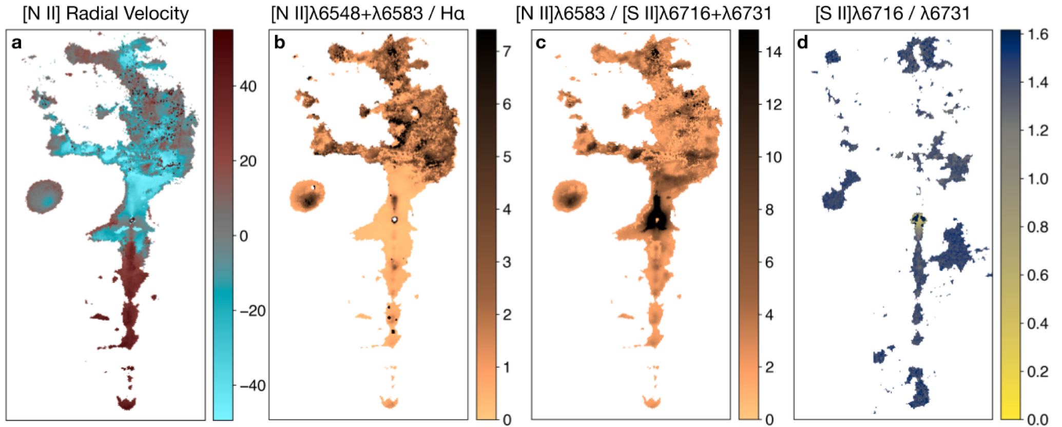
Figure 4. from Janette Suherli et al 2026 Astrophys. J. Lett. 997 doi:10.3847/2041-8213/ae27c4 https://dx.doi.org/10.3847/2041-8213/ae27c4 © 2026. The Author(s). Published by the American Astronomical Society.
