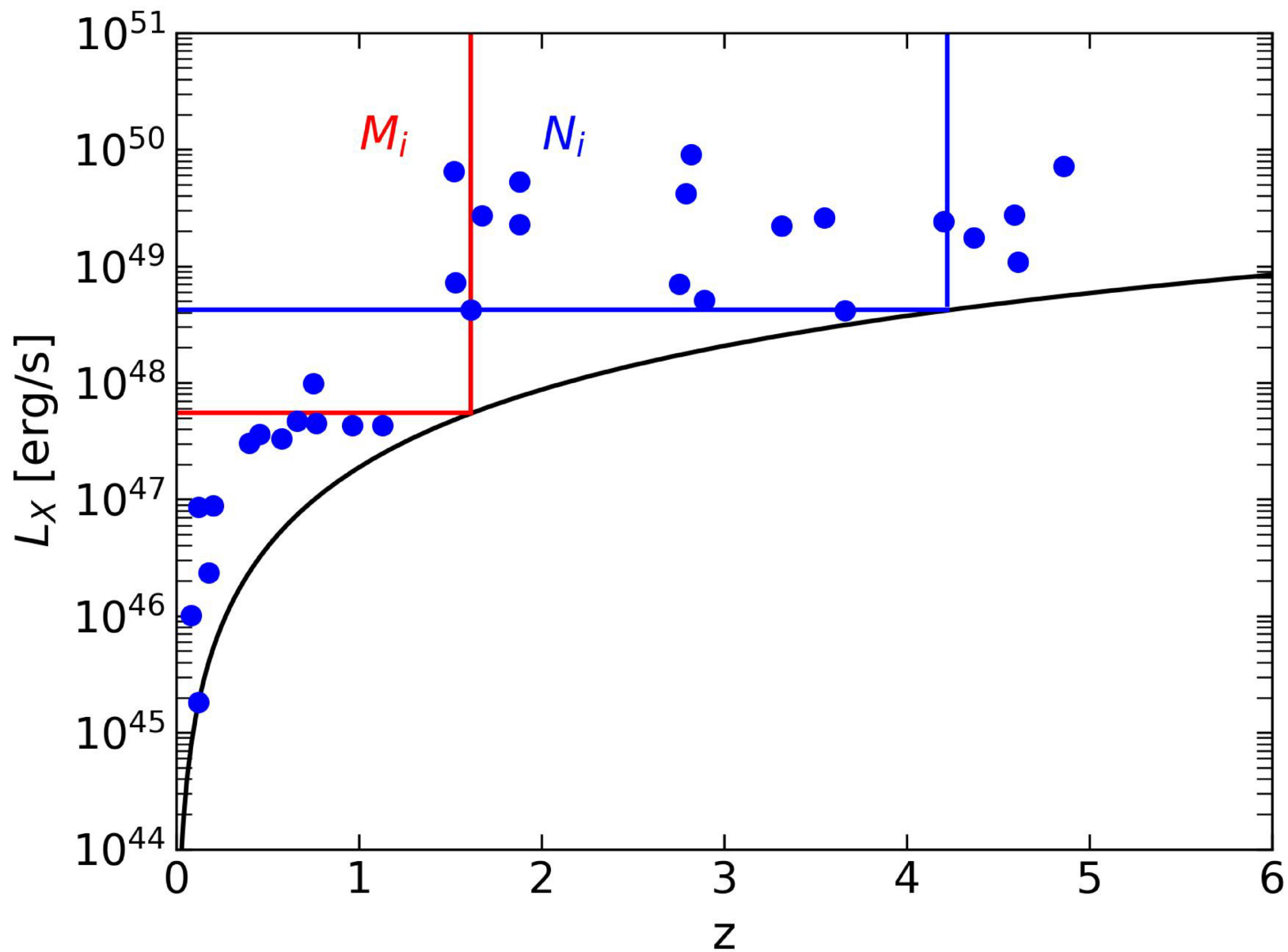
Figure 1. from Yizhou Guo et al 2025 Astrophys. J. Lett. 995 doi:10.3847/2041-8213/ae2745 https://dx.doi.org/10.3847/2041-8213/ae2745 © 2025. The Author(s). Published by the American Astronomical Society.
