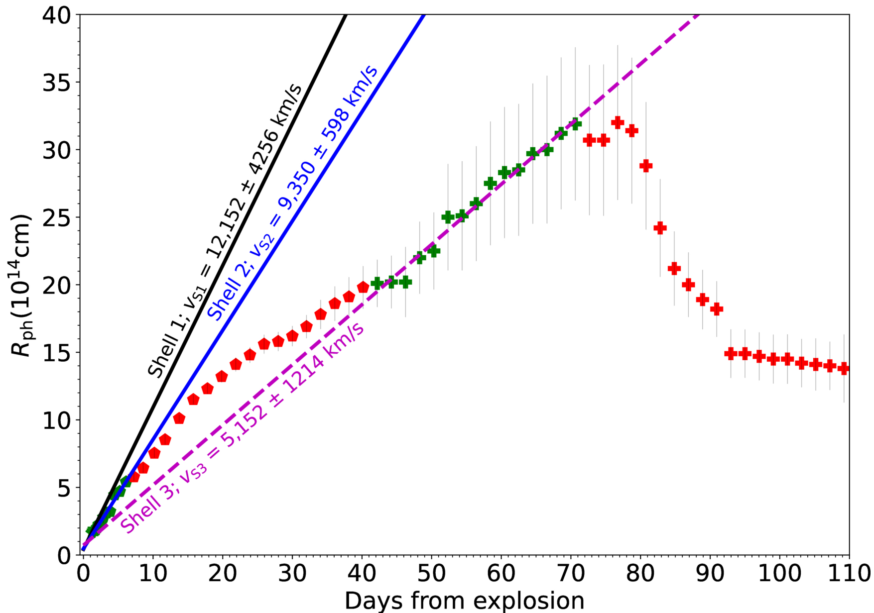
Figure 2. from Noam Soker and Kobi Shiran 2025 Astrophys. J. Lett. 995 doi:10.3847/2041-8213/ae21da https://dx.doi.org/10.3847/2041-8213/ae21da © 2025. The Author(s). Published by the American Astronomical Society.
