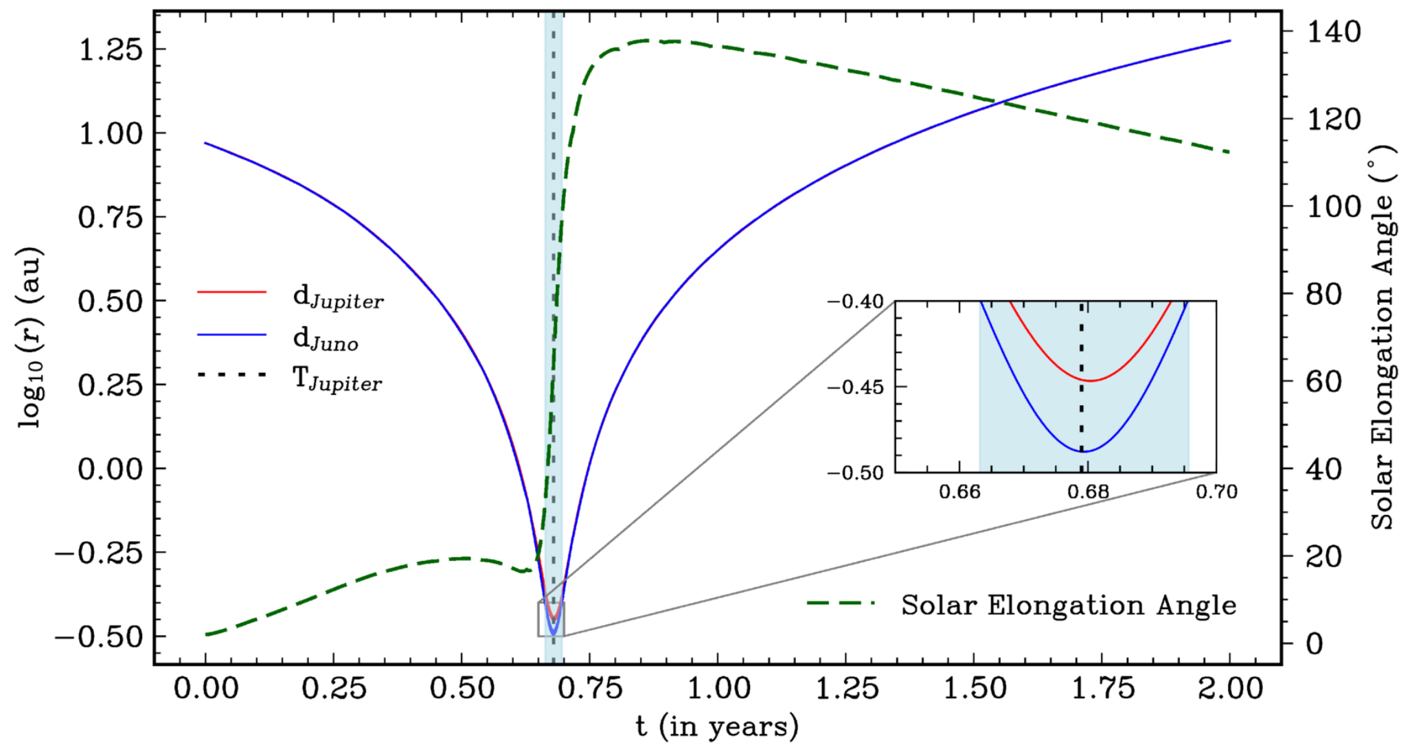
Figure 3. from Goldy Ahuja and Shashikiran Ganesh 2025 Astrophys. J. Lett. 995 doi:10.3847/2041-8213/ae21cf https://dx.doi.org/10.3847/2041-8213/ae21cf © 2025. The Author(s). Published by the American Astronomical Society.
