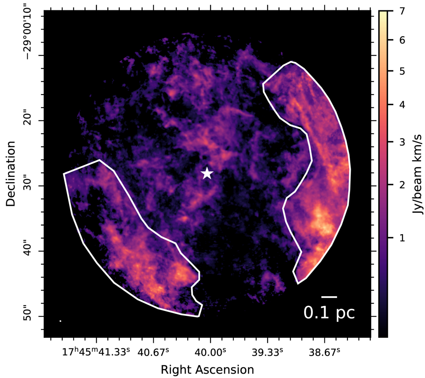
Figure 1. from Mark D. Gorski and Lena Murchikova 2025 Astrophys. J. Lett. 995 doi:10.3847/2041-8213/ae211f https://dx.doi.org/10.3847/2041-8213/ae211f © 2025. The Author(s). Published by the American Astronomical Society.
