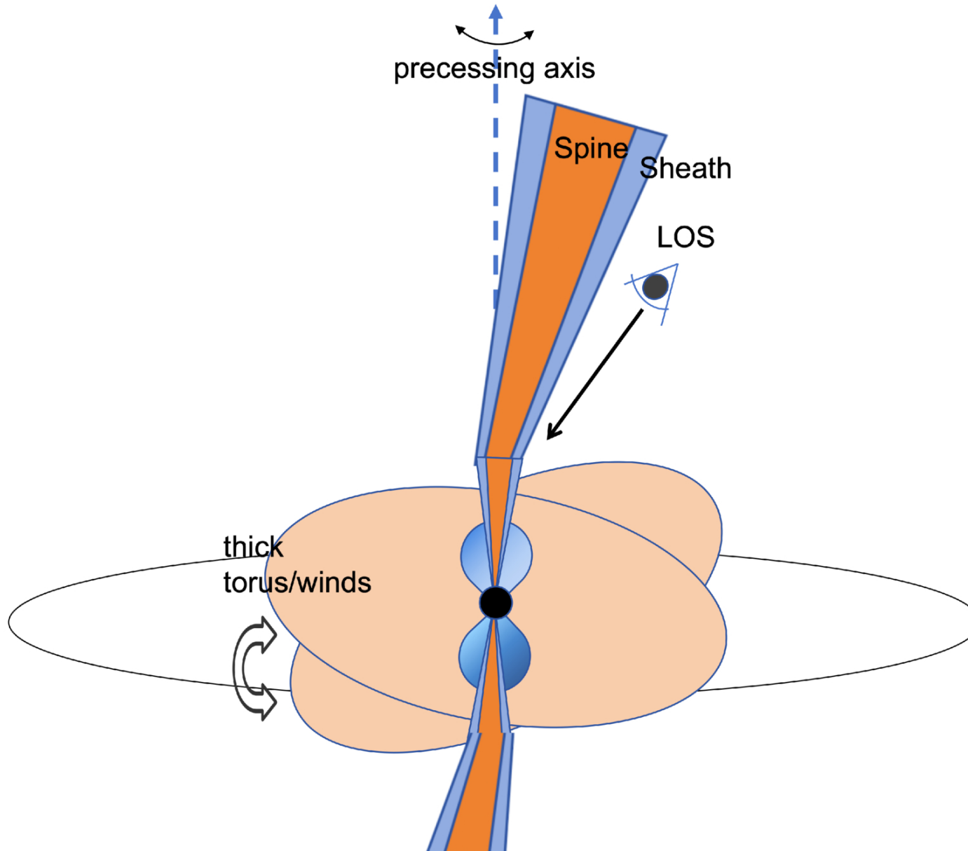
Figure 1. from Tao An 2025 Astrophys. J. Lett. 995 doi:10.3847/2041-8213/ae2028 https://dx.doi.org/10.3847/2041-8213/ae2028 © 2025. The Author(s). Published by the American Astronomical Society.
