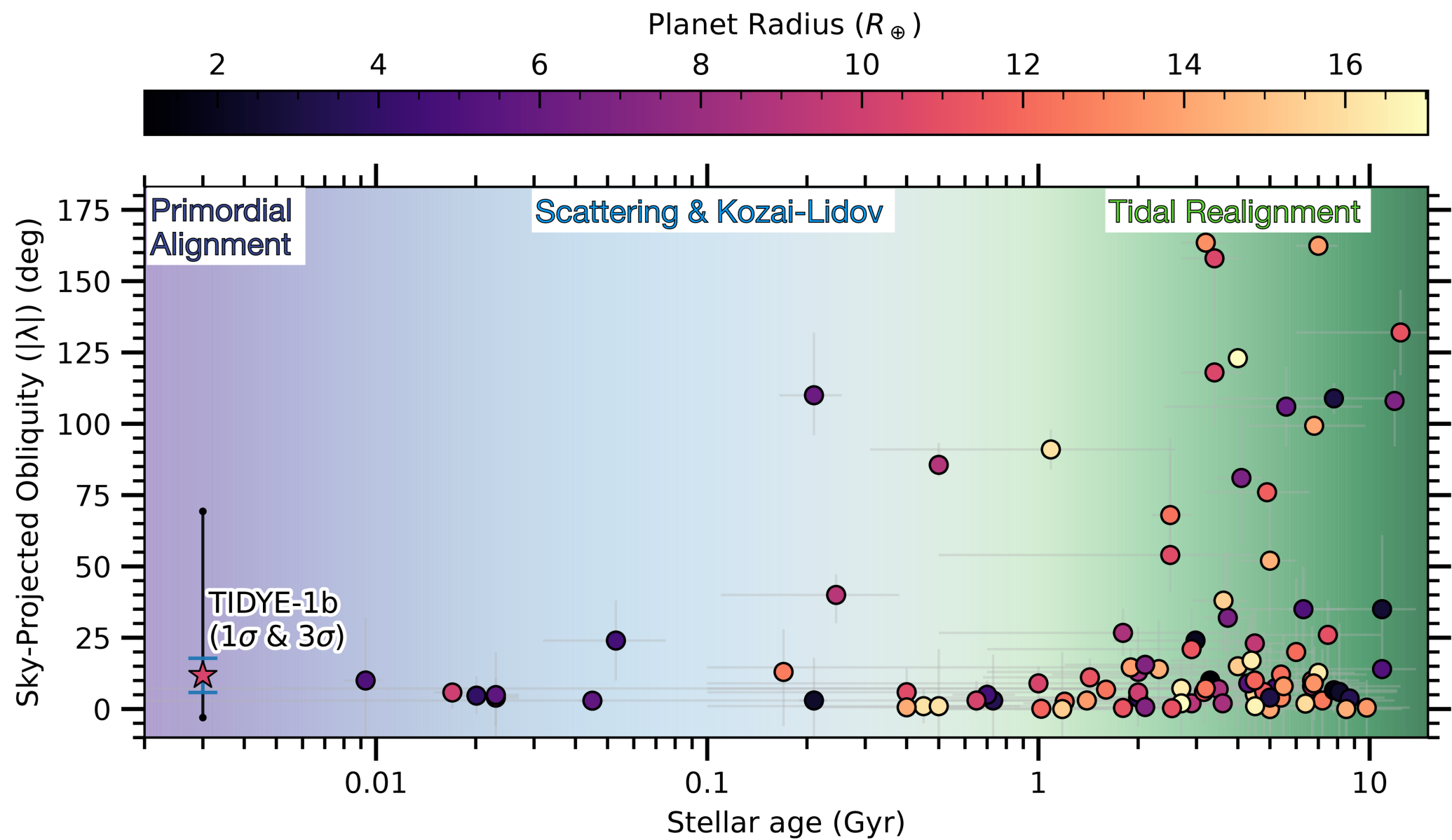
Figure 4. from Madysen G. Barber et al 2025 Astrophys. J. Lett. 994 doi:10.3847/2041-8213/ae2004 https://dx.doi.org/10.3847/2041-8213/ae2004 © 2025. The Author(s). Published by the American Astronomical Society.
