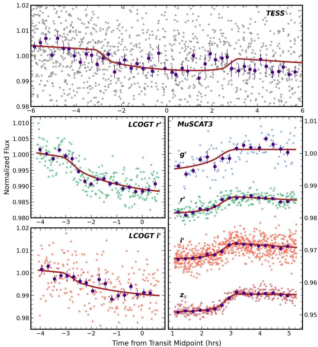
Figure 1. from Madysen G. Barber et al 2025 Astrophys. J. Lett. 994 doi:10.3847/2041-8213/ae2004 https://dx.doi.org/10.3847/2041-8213/ae2004 © 2025. The Author(s). Published by the American Astronomical Society.
