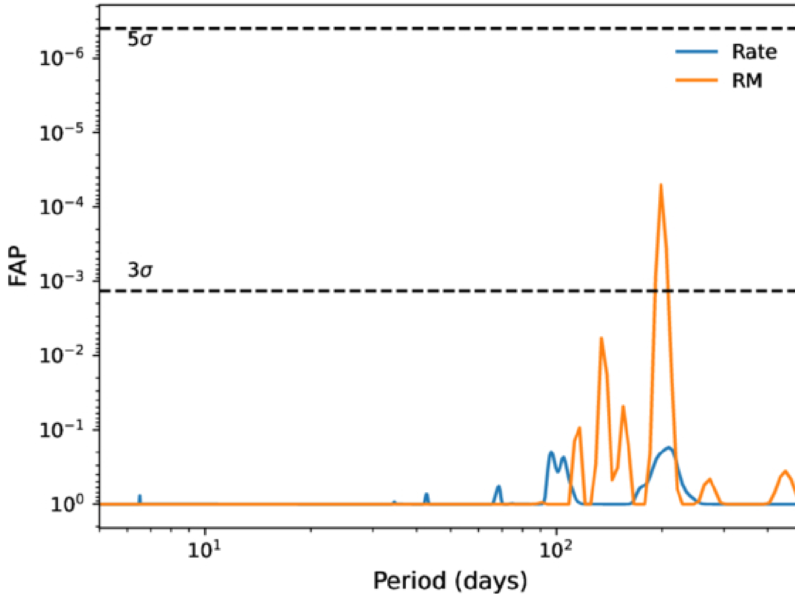
Figure 5. from Yi-Fang Liang et al 2025 Astrophys. J. Lett. 994 doi:10.3847/2041-8213/ae1d60 https://dx.doi.org/10.3847/2041-8213/ae1d60 © 2025. The Author(s). Published by the American Astronomical Society.
