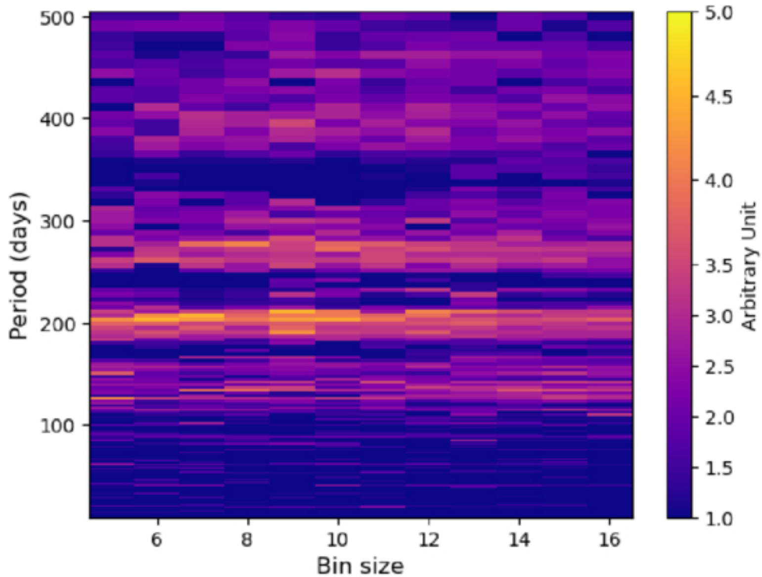
Figure 4. from Yi-Fang Liang et al 2025 Astrophys. J. Lett. 994 doi:10.3847/2041-8213/ae1d60 https://dx.doi.org/10.3847/2041-8213/ae1d60 © 2025. The Author(s). Published by the American Astronomical Society.
