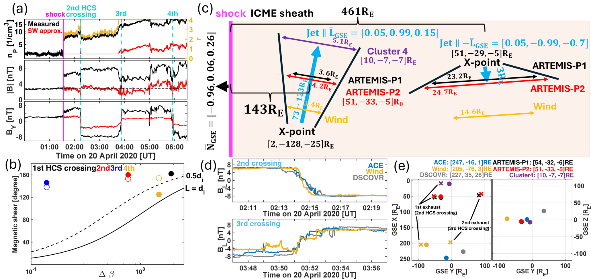
Figure 4. from Matti Ala-Lahti et al 2025 Astrophys. J. Lett. 994 doi:10.3847/2041-8213/ae1d44 https://dx.doi.org/10.3847/2041-8213/ae1d44 © 2025. The Author(s). Published by the American Astronomical Society.
