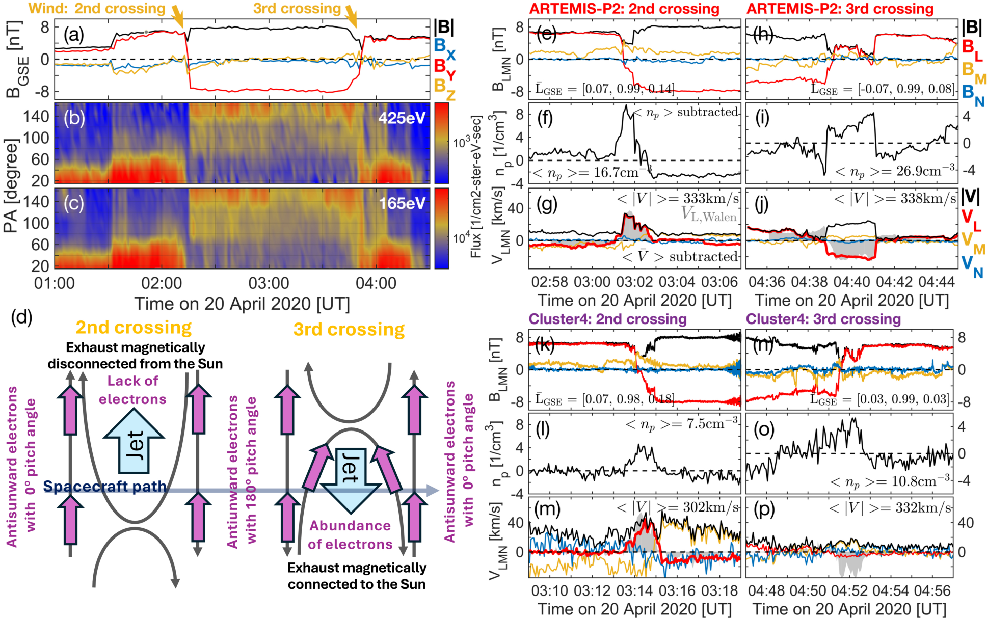
Figure 3. from Matti Ala-Lahti et al 2025 Astrophys. J. Lett. 994 doi:10.3847/2041-8213/ae1d44 https://dx.doi.org/10.3847/2041-8213/ae1d44 © 2025. The Author(s). Published by the American Astronomical Society.
