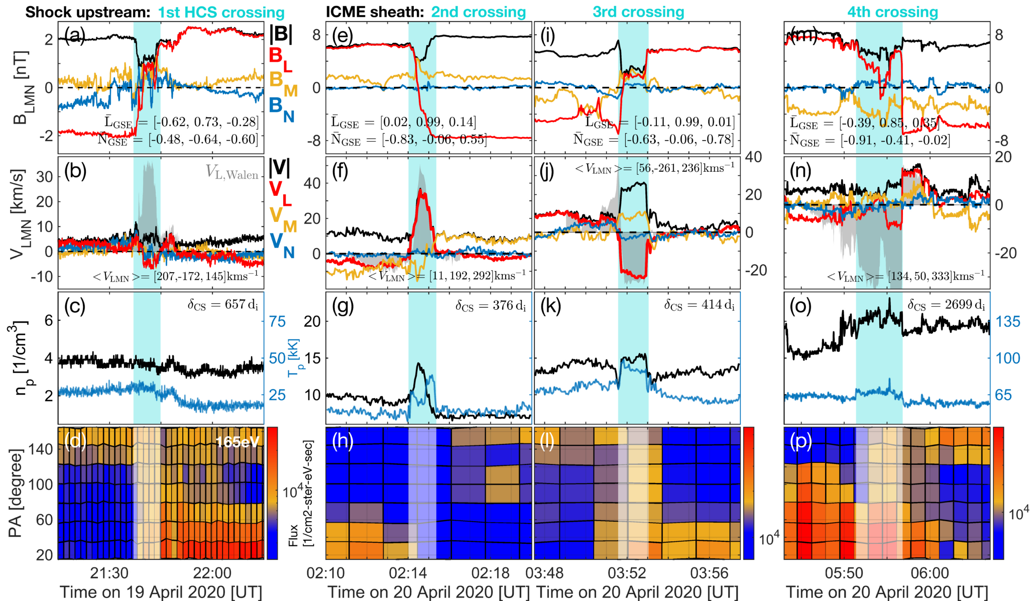
Figure 2. from Matti Ala-Lahti et al 2025 Astrophys. J. Lett. 994 doi:10.3847/2041-8213/ae1d44 https://dx.doi.org/10.3847/2041-8213/ae1d44 © 2025. The Author(s). Published by the American Astronomical Society.
