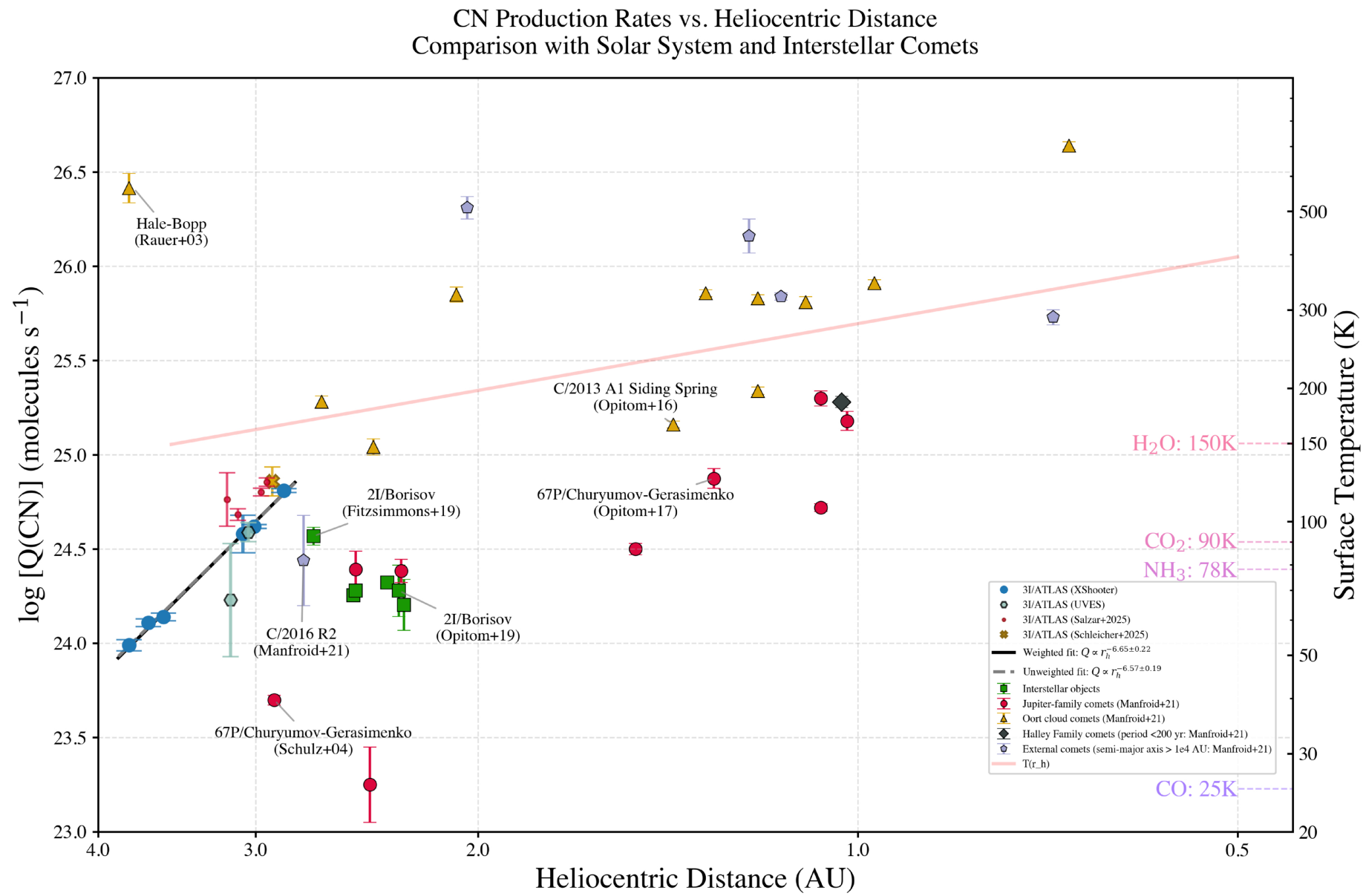
Figure 4. from Rohan Rahatgaonkar et al 2025 Astrophys. J. Lett. 995 doi:10.3847/2041-8213/ae1cbc https://dx.doi.org/10.3847/2041-8213/ae1cbc © 2025. The Author(s). Published by the American Astronomical Society.
